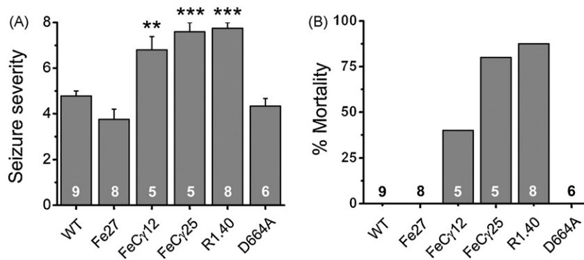
Fig. 2. Increased seizure susceptibility to kainic acid in FeC \gamma and R1.40 mice. (A) Quantification of maximum seizure severity exhibited over a 65 min monitoring period in mice of the indicated lines injected i.p. with kainic acid. (B) Percent mortality during the monitoring period after kainic acid injection. Data expressed as \pm SEM, ** p < 0.01, *** p < 0.001 (one way ANOVA, Bonferroni's post-test).
