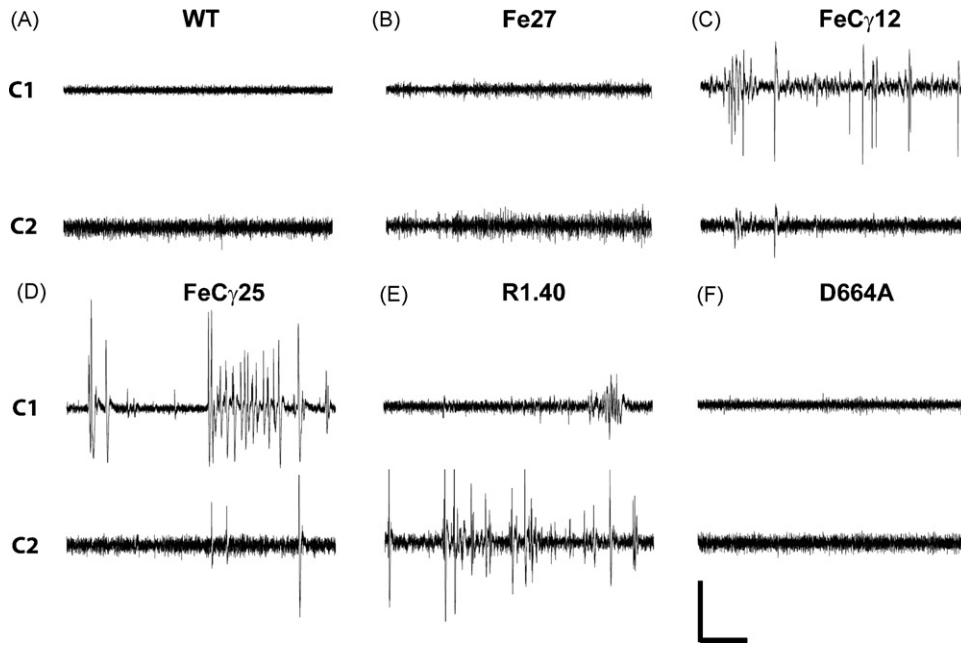
Fig. 1. Abnormal EEG episodes in AICD/Fe65 and R1.40 mice. Representative EEG rhythms in WT mice (12 of 12) (A) and Fe27 mice (6 of 7) (B). Representative EEGs from abnormal spiking periods in FeC \gamma 12 (7 of 8) (C), FeC \gamma 25 (7 of 7) (D), and R1.40 mice (6 of 6) (E). Representative EEG trace from PDAPP(D664A) mice (4 of 5) (F). Scale bar in (F): vertical 100 \mu A, horizontal 20 s. C1: EEG channel one: parietal cortex and C2: EEG channel two: frontal-parietal cortices.
